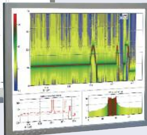
Spectrogram
